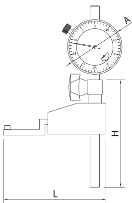
Centre Align Dial ● 5671-0015 Used to adjust the concentricity of cylinder bore and bore bar
